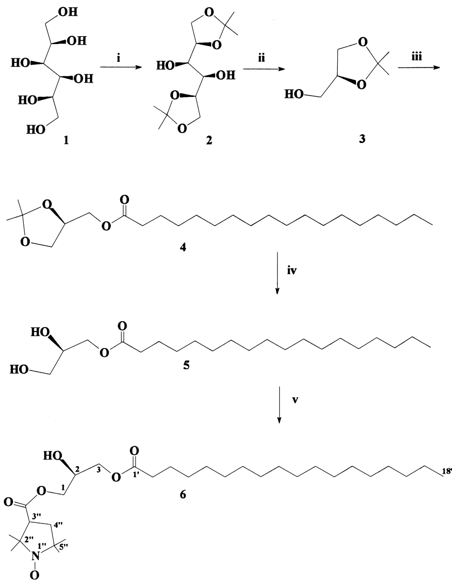
Scheme 1. Synthesis of 1-[2-hydroxy-3-octadecan-1'-oate]propyl-2'',2'',5'',5''-tetramethyl pyrrolidine- N -oxyl-3''-carboxylate ( 6 ). Conditions: (i) acetone, \text{ZnCl}_2 , \text{K}_2\text{CO}_3 ; (ii) \text{NaIO}_4 , \text{NaBH}_4 ; (iii) stearic acid, DMAP, DCC; THF; (iv) Dowex 50W \times 8; (v) 3-carboxy proxyl, DCC, DMAP, THF, 16 h.
