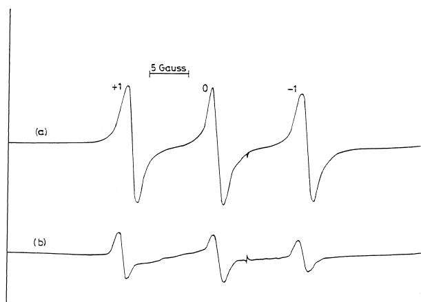
Figure 1. ESR spectra of the nitroxide 6 in (a) solution state ( \text{CHCl}_3 ) and (b) DPPC liposomes.
