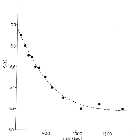
Figure 3. Plot of time (s) vs the signal height S(t) of the ESR spectrum of the spin label 7 incorporated into DPPC liposomes in the presence of epinephrine.
