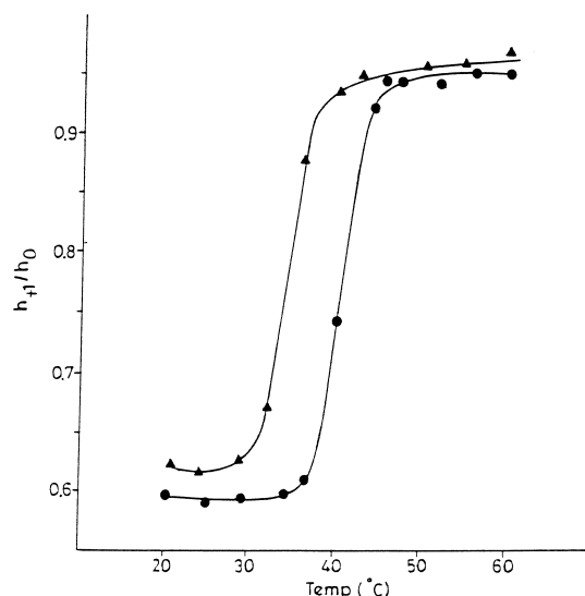
Figure 2. Plot of temperature (°C) vs spectral parameter h_{+1}/h_0 of the spin label 6 incorporated into pure DPPC liposomes (●) and in the presence of diltiazem (▲).
